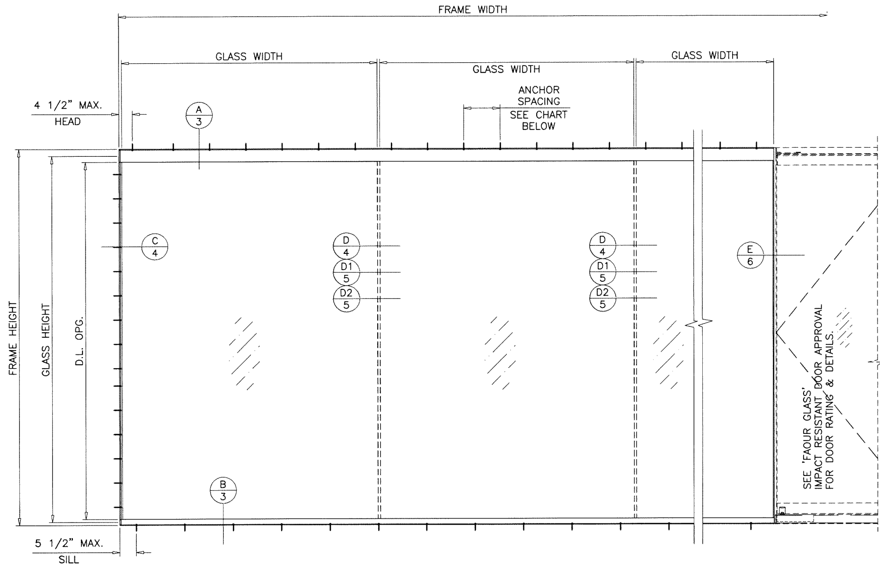
TYPICAL ELEVATIONS
